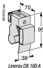
Linergy DX 160 А
