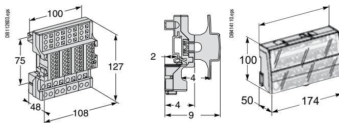
Linergy DX 125 и 160 A
